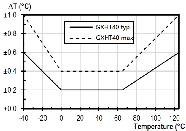
Figure 8 GXHT40 temperature accuracy
